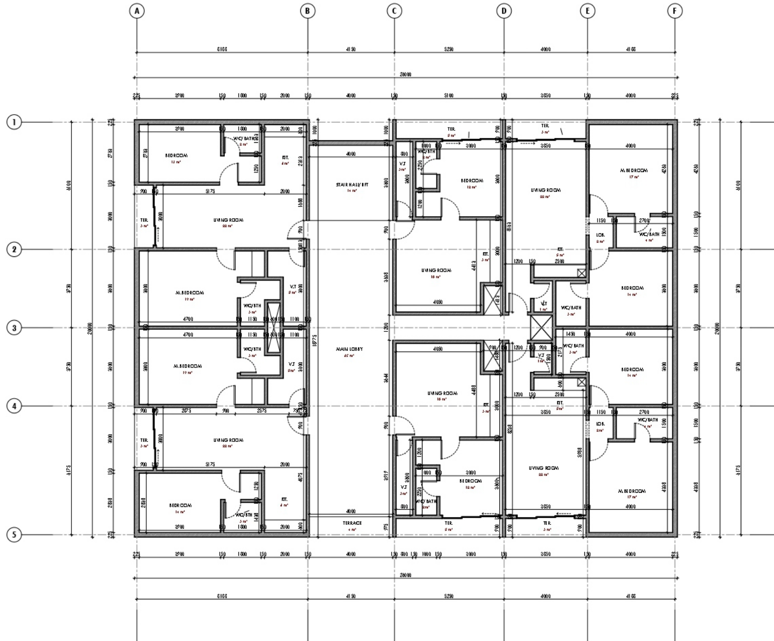
TYPICAL FIRST/SECOND/THIRD FLOOR PLAN
